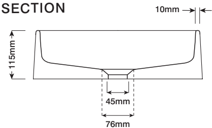
CROSS SECTION
