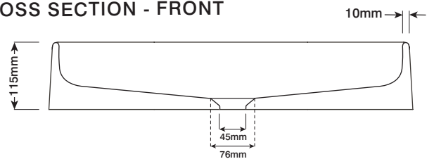
CROSS SECTION - FRONT
