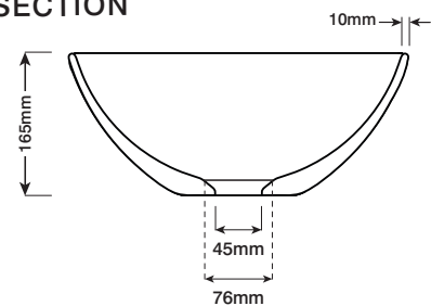
CROSS SECTION
